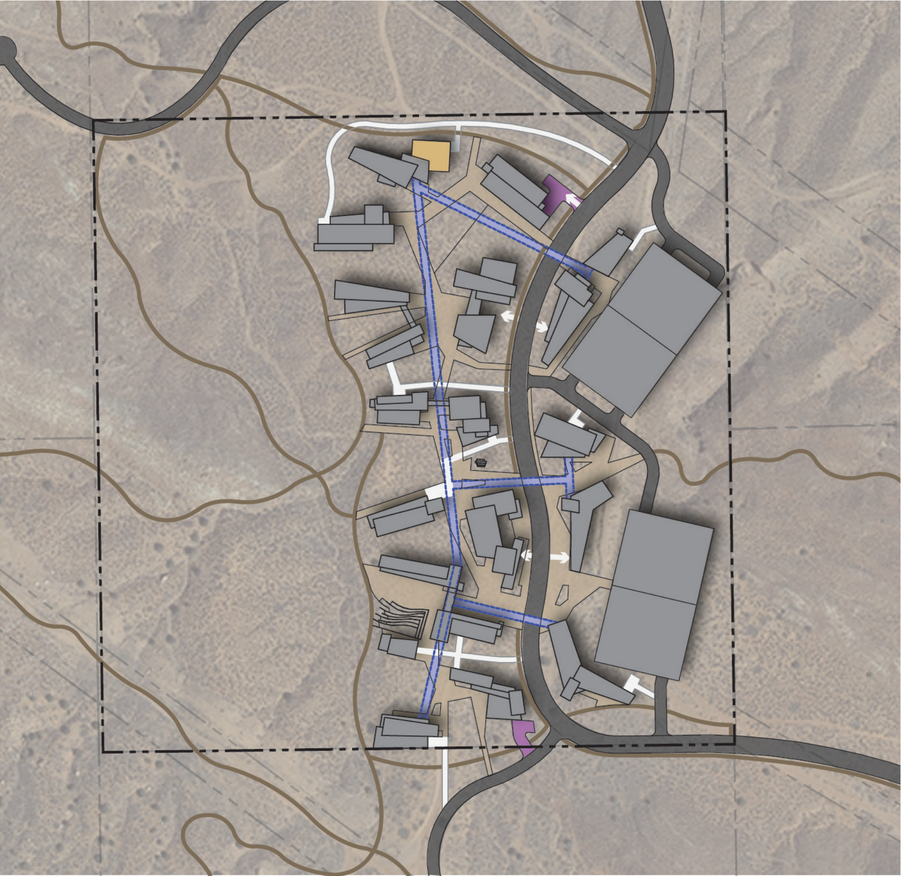
CAMPUS UTILITIES AND SERVICE DIAGRAM
