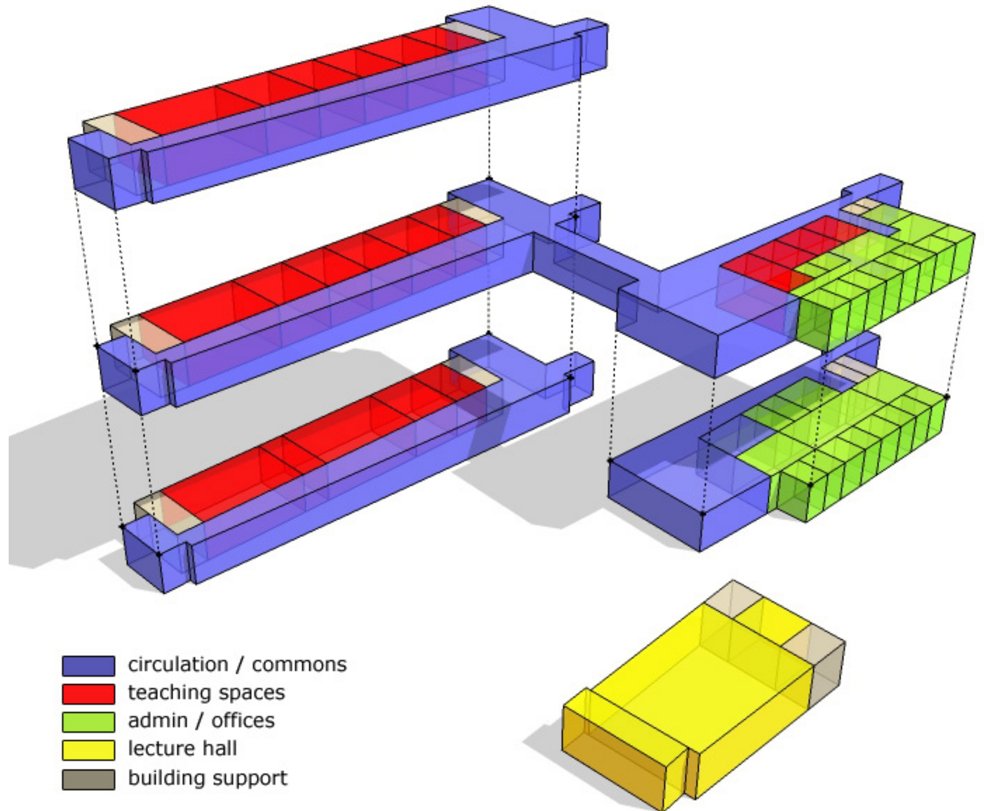
MASSING DIAGRAM
