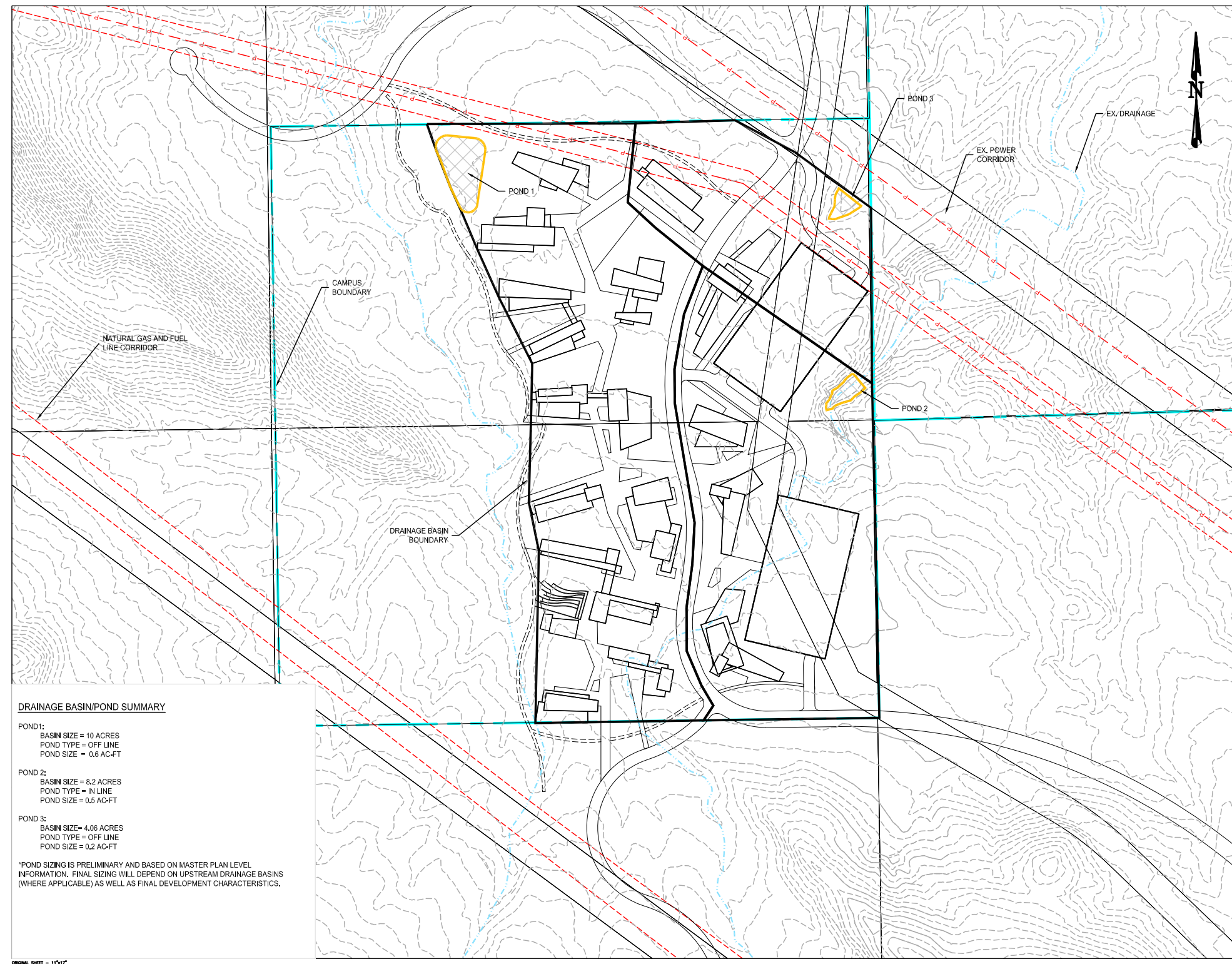
FIGURE UT-3: STORM WATER SYSTEM FRAMEWORK
