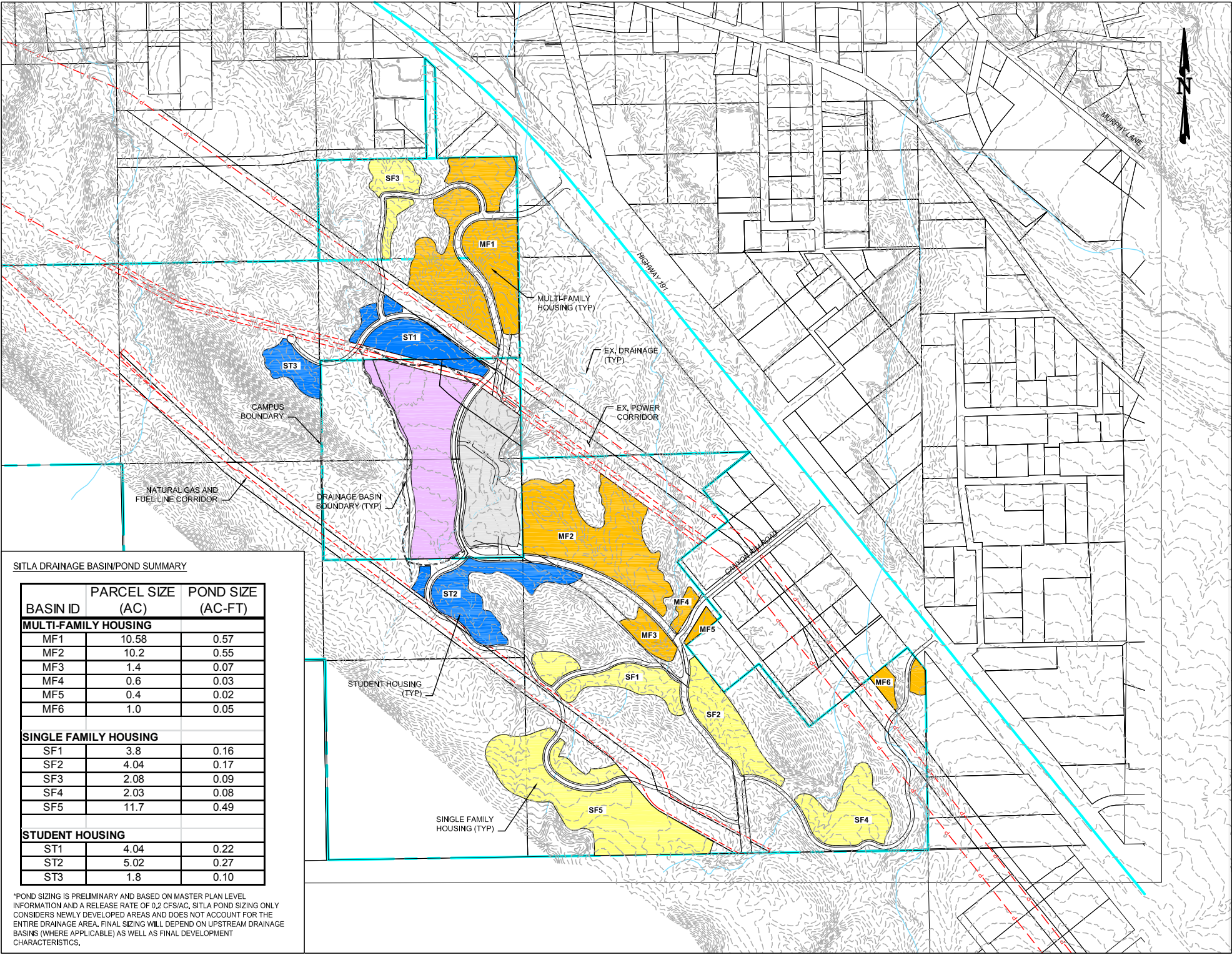
FIGURE UT-3B: STORM WATER SYSTEM FRAMEWORK
